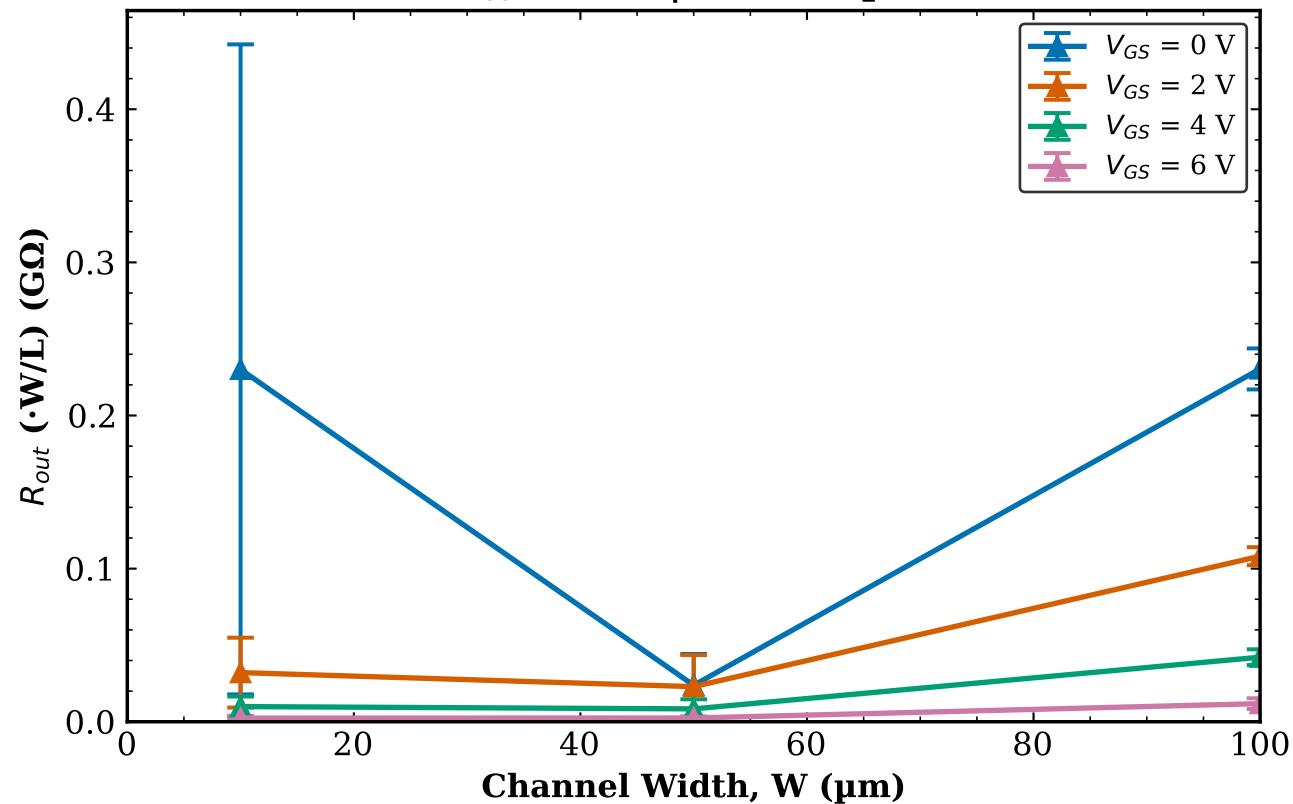
TFT3 Combined (Tr. 1 & 2) R_{out} vs W | L = 20\text{ }\mu\text{m}
